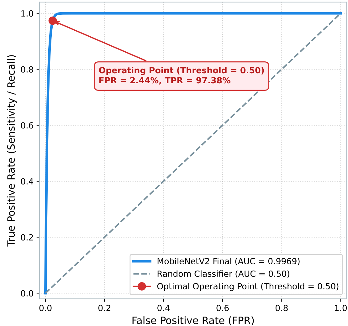
Figure 4(b): Receiver Operating Characteristic (ROC) (Confirming Near-Perfect Class Discrimination)
