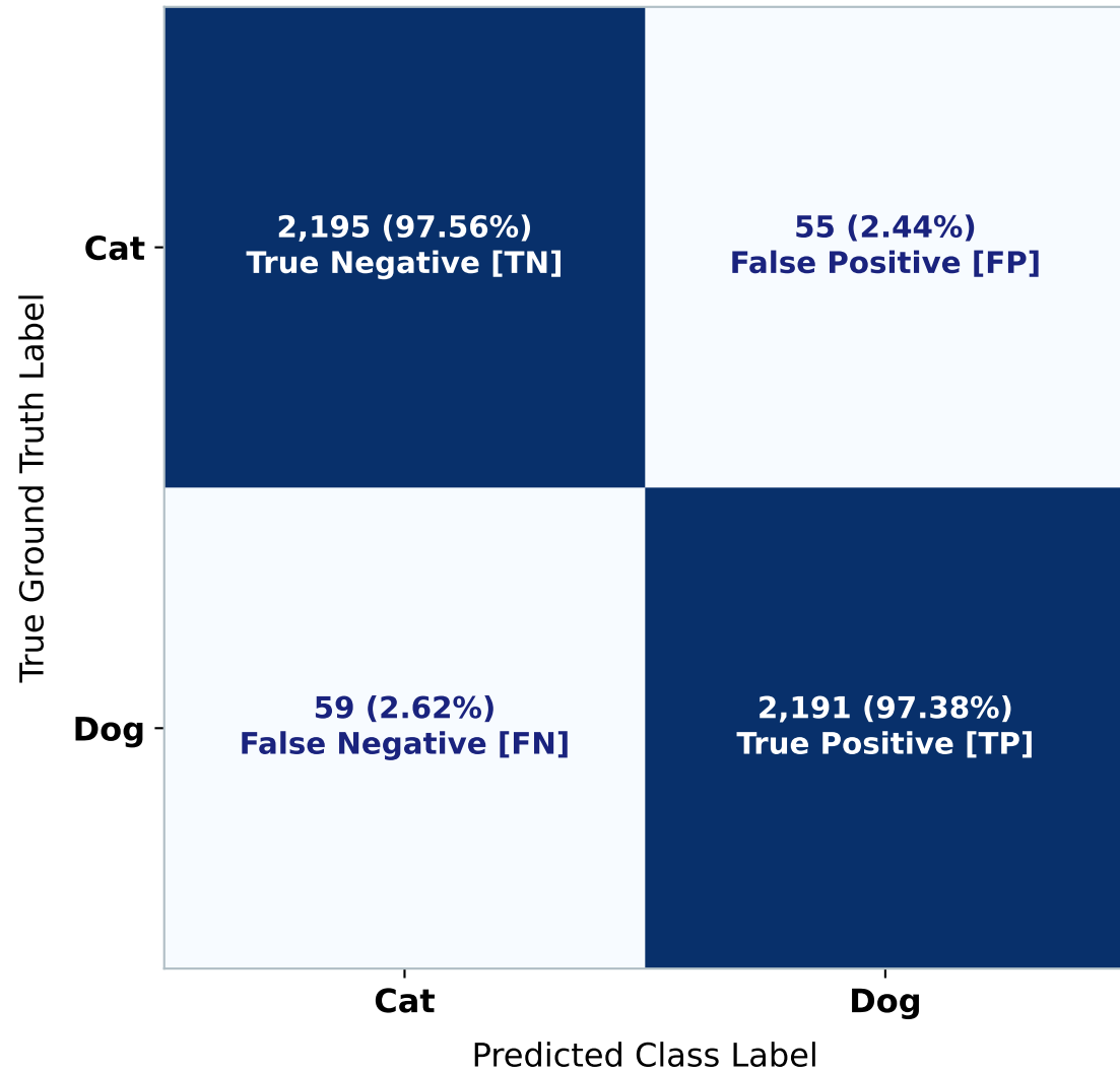
Figure 4(a): Normalized Confusion Matrix (Validation Holdout Set, N = 4,500 Images)
