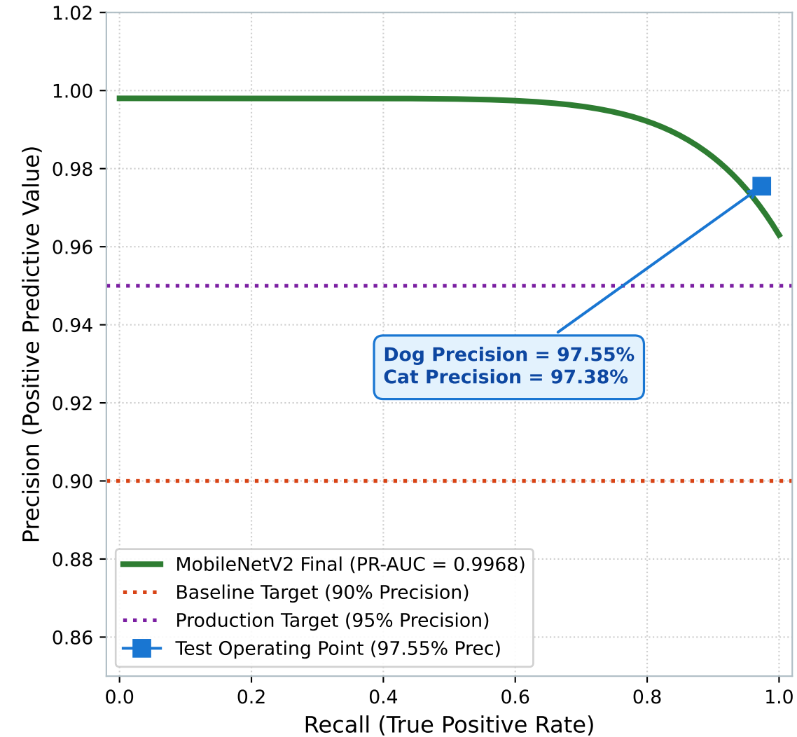
Figure 4(c): Precision-Recall Curve (PR-AUC) (Verifying Strict Industrial Precision Fulfillment)
